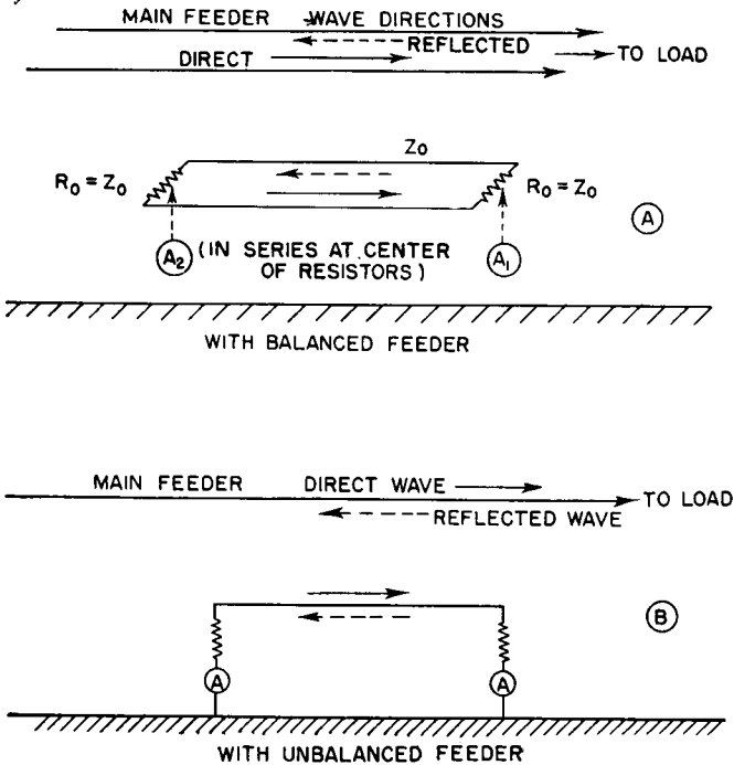
Fig. 4.62. Standing-wave indicators.
