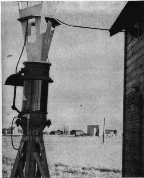
FIG. 2.64. Base insulator of the Austin oil-filled safety-core type with the tower-lighting transformer inside the base insulator, at Station CKLW. (Photograph courtesy of RCA Victor Company, Ltd., Montreal.)
