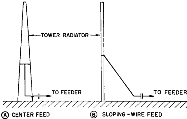
FIG. 2.8. Shunt-fed vertical radiators.
