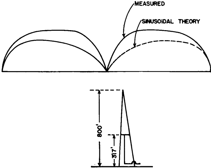
FIG. 2.11. Measured vertical patterns for axial shunt-fed vertical radiator.
