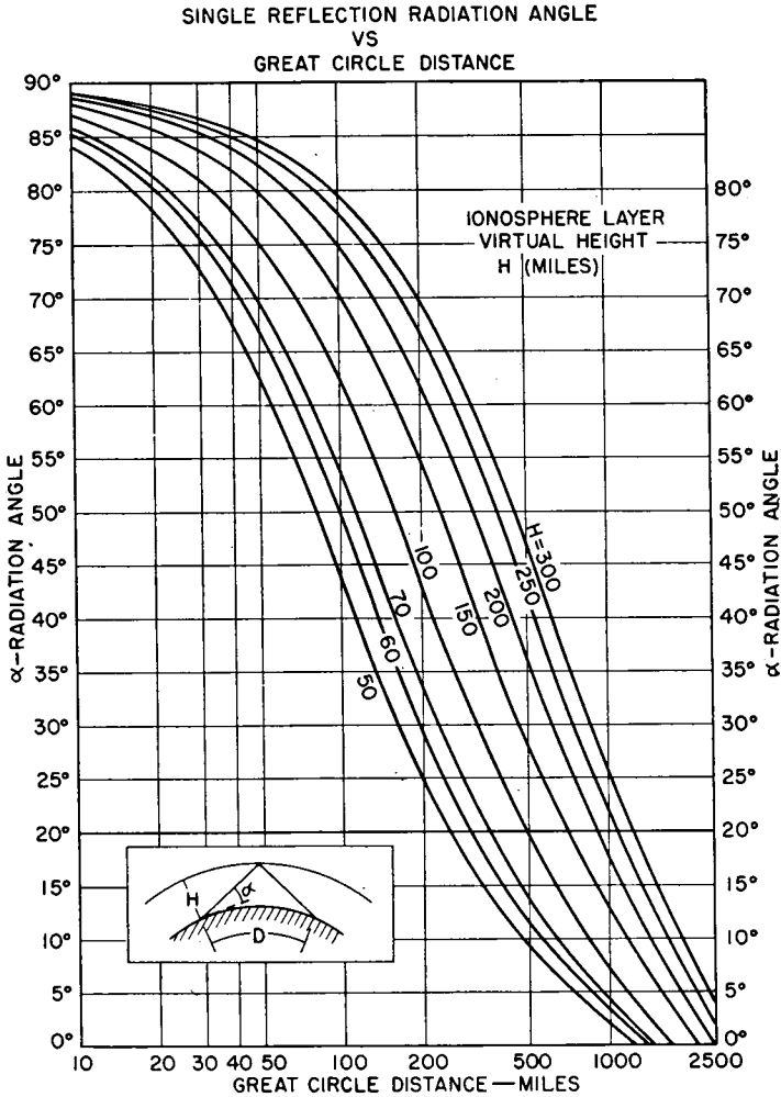
Fig. 2.3. Vertical radiation angles for sky-wave propagation.
