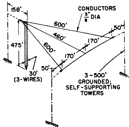
FIG. 1.29. Single-tuned inverted-L antenna with horizontal portion expanded.
