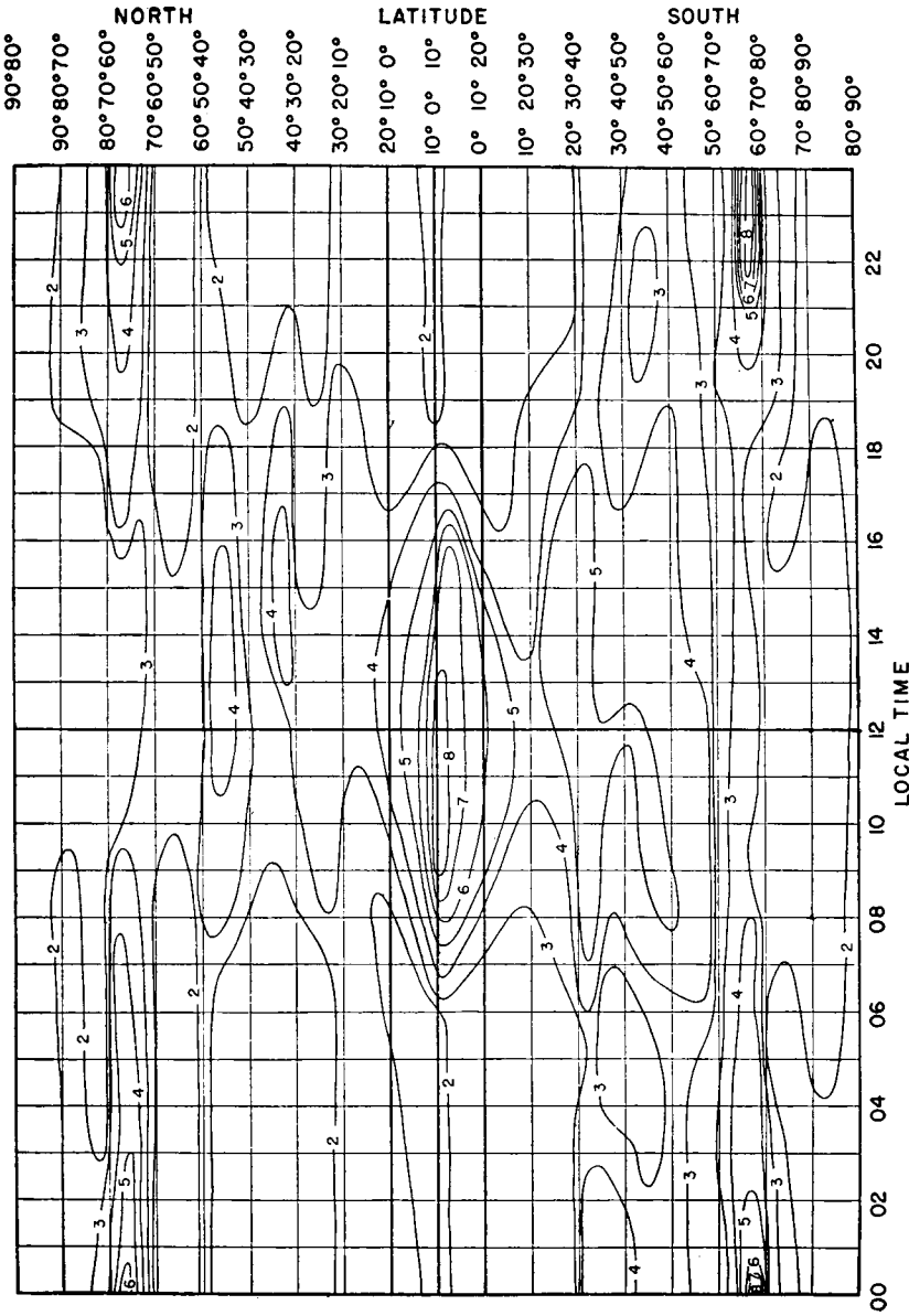
FIG. 3.5. Median E sporadic, in megacycles, predicted for January, 1947. (After Central Radio Propagation Laboratory.)
