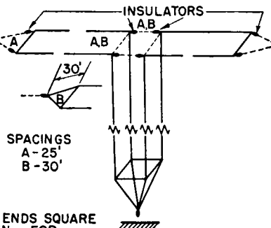
Fig. 1.31. Two-wire T antenna.
