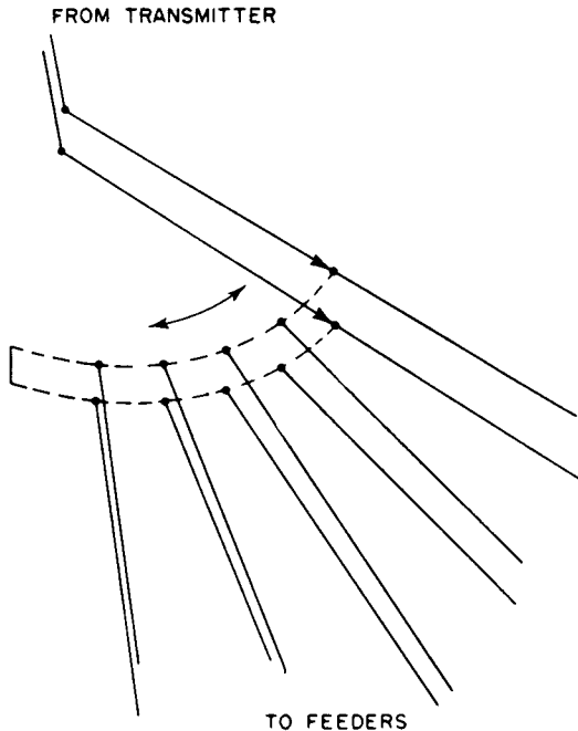
FIG. 4.55. Multiposition switch.
