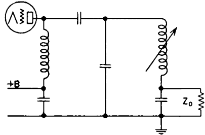
FIG. 4.33. Transmitter output-coupling circuit.
