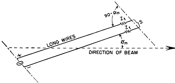
FIG. 3.72. Elementary two-wire traveling-wave antenna.
