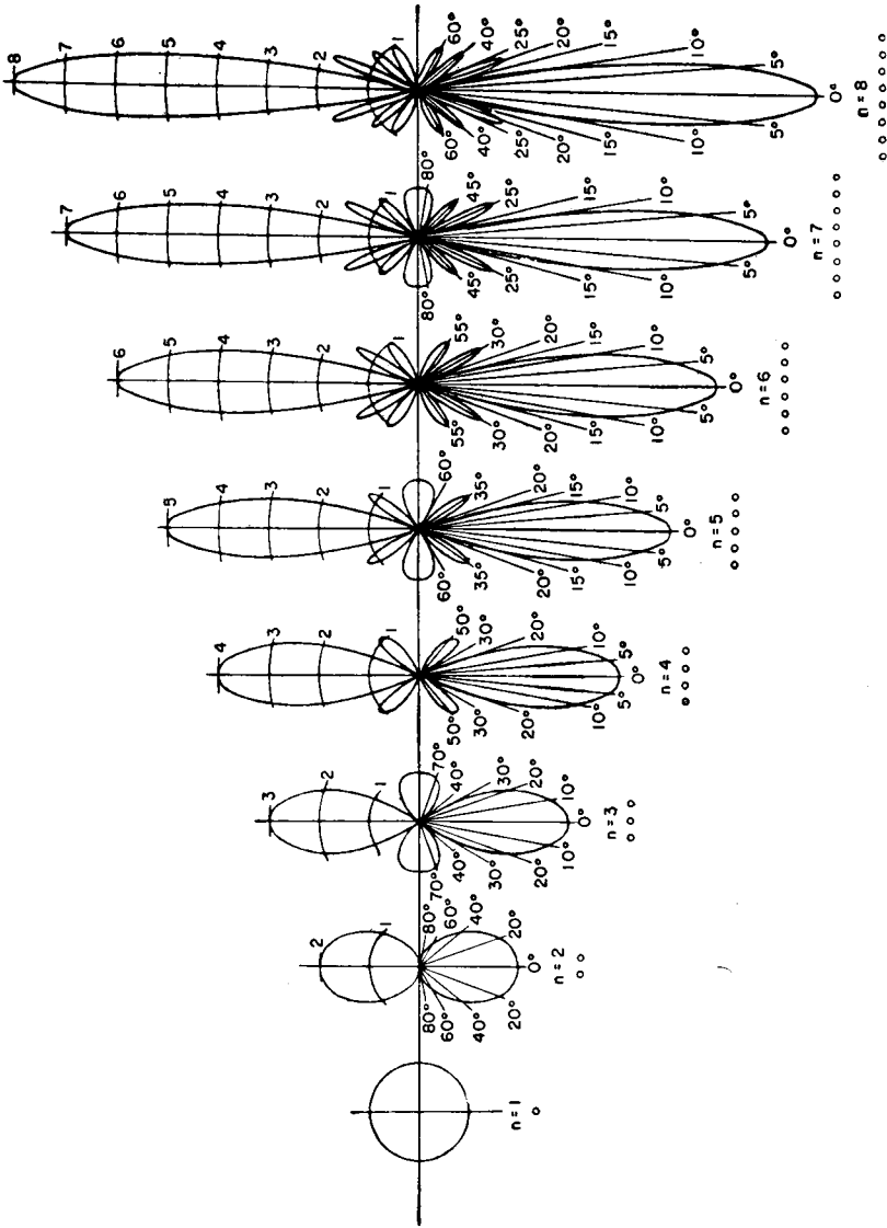
FIG. 3.46. Radiation patterns for horizontal row of vertical dipoles with unit current, cophased. (From RAF Signal Manual.)
