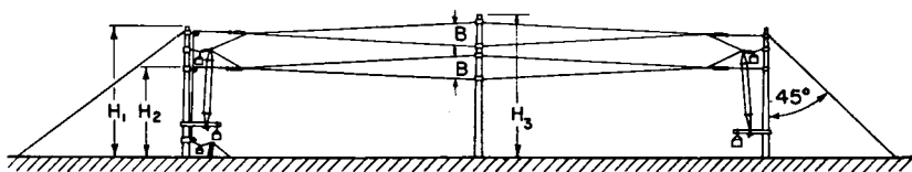
SIDE ELEVATION
